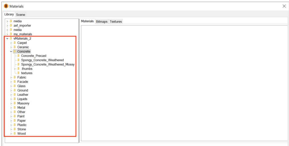
Fig. 3.2 – Library treeview
