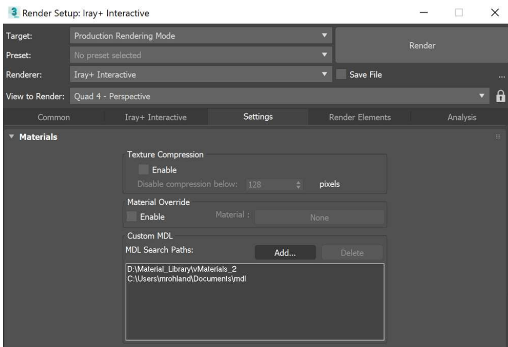
Fig. 3.3 – Defining the location of the vMaterials
