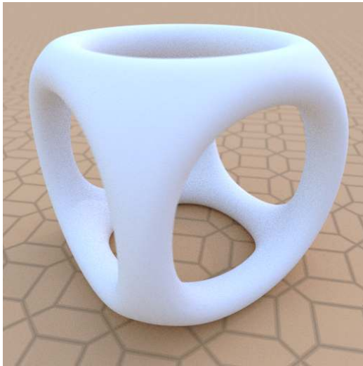
Fig. 5.1 - diffuse_reflection_bsdf
