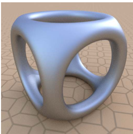
Fig. 5.6 - simple_glossy_bsf
