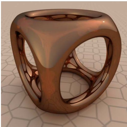
Fig. 5.5 - specular_bsf
