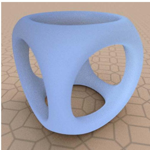
Fig. 5.7 - backscattering_glossy_reflection_bsf
