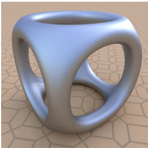
Fig. 5.6 - simple_glossy_bsdf
