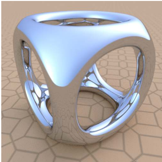
Fig. 5.3 - specular_bsdf
