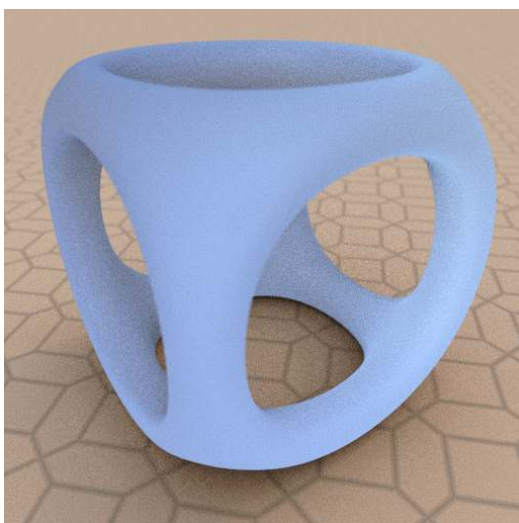
Fig. 5.7 - backscattering_glossy_reflection_bsdf
