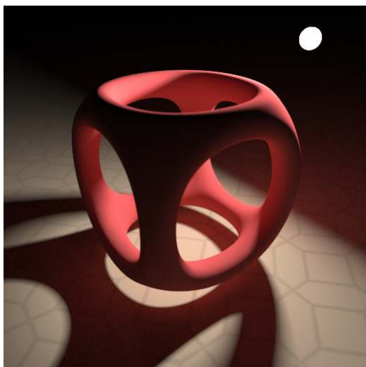
Fig. 5.10 - measured_edf
